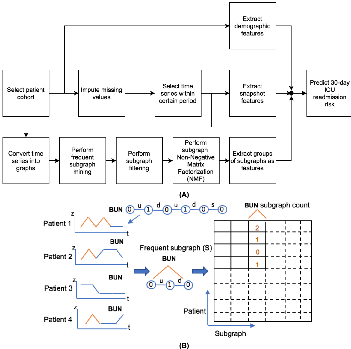
Fig. 1. (A) The flowchart of proposed approach, moving from selecting data to predicting readmission risk. (B) An example of creating a matrix of common subgraphs. Only the Blood Urea Nitrogen (BUN) trend graph for patient 1 is shown (BUN 0 1 0 1 0 0). The frequent subgraph is (BUN 0-u-1-d-0), noted as S. Patient 1 has two frequent subgraphs S; patients 2 and 4 have one; and patient 3 has no S. The edge labels, "u," "d" and "s," are short for "up," "down" and "same," respectively.
