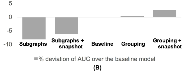
Fig. 2. (A) ROC curves of different ICU readmission risk predictive models. (B) Percentage deviation of AUC over the baseline model.
